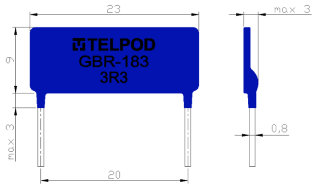
Fig. 1. Preview with dimensions [mm]
